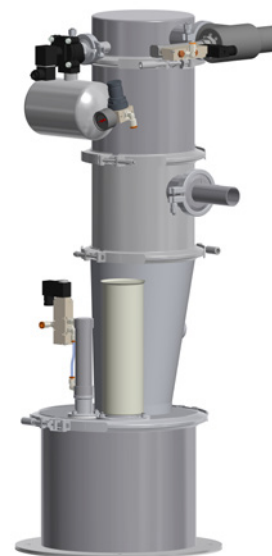
P10 receiver with powered flap valve
